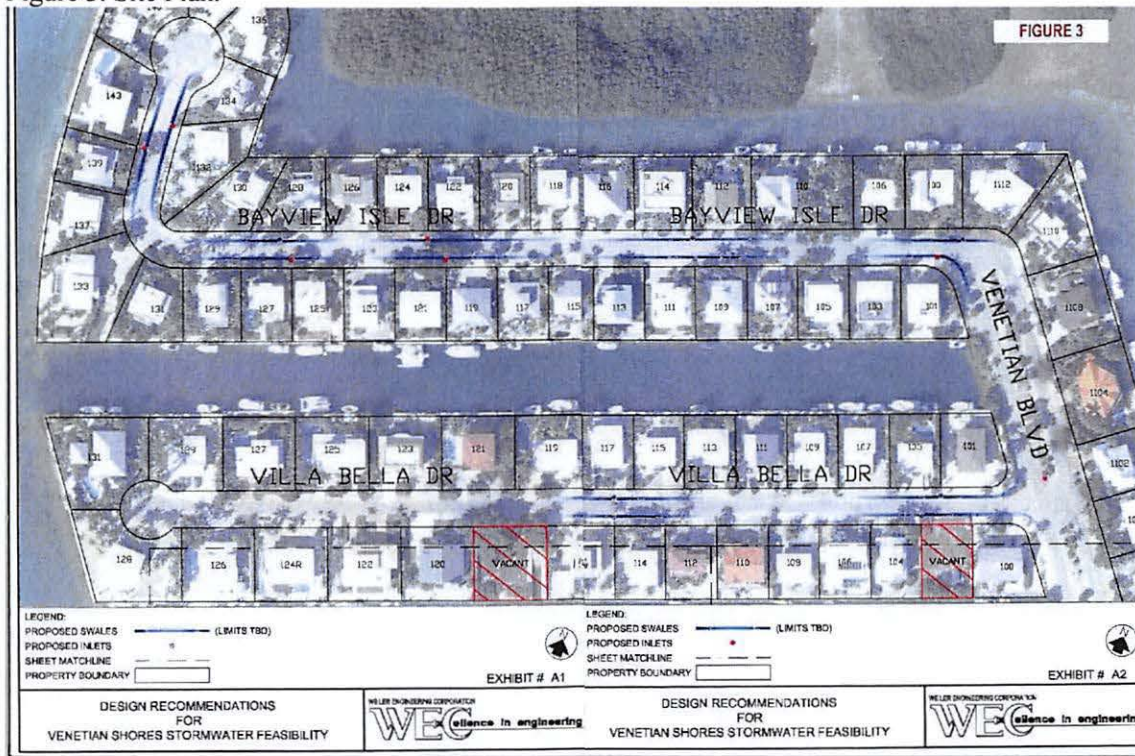
Figure 3. Site Plan.
